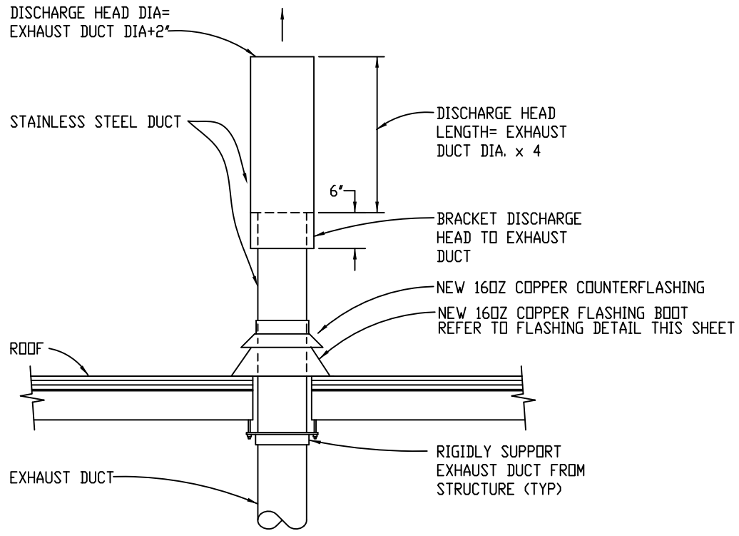
EXHAUST STACK DISCHARGE HEAD DETAIL NO SCALE
